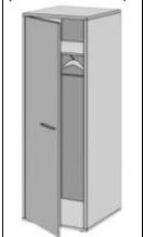
ДБ99 (ДБ99_1 + ДБ99_2) (550x400x1980)
